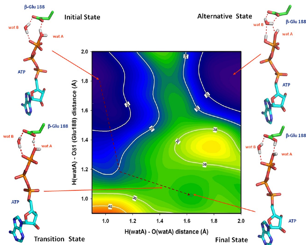
Figure 3. Free energy landscape for the activation of the catalytic water molecule assuming \beta -Glu 188 is the proton acceptor. \Delta G_0 values obtained for the whole system are shown for the different states corresponding to the distances: x axis, from the proton to the oxygen atom in the active water molecule (wat A); y axis, from the same proton to O \delta 1 of \beta -Glu 188. The structure of the active center is depicted in the initial, transition, and two alternative final states. In all cases, the \gamma -phosphate group of ATP exhibited a pentacovalent conformation.
